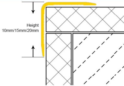
Aluminium Tile Trims
