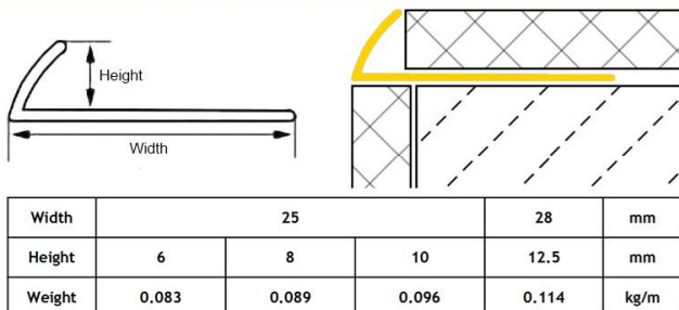
Aluminium Tile Trims
